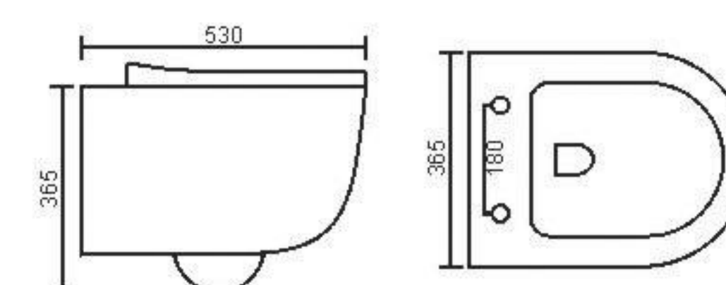
MUSTANG TORNADO Wall Hun WC
