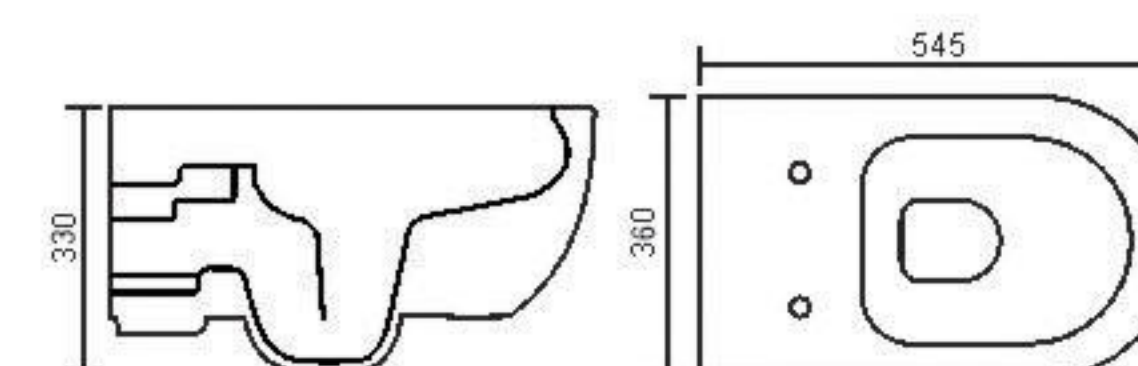
NICOLA Wall Hung WC
