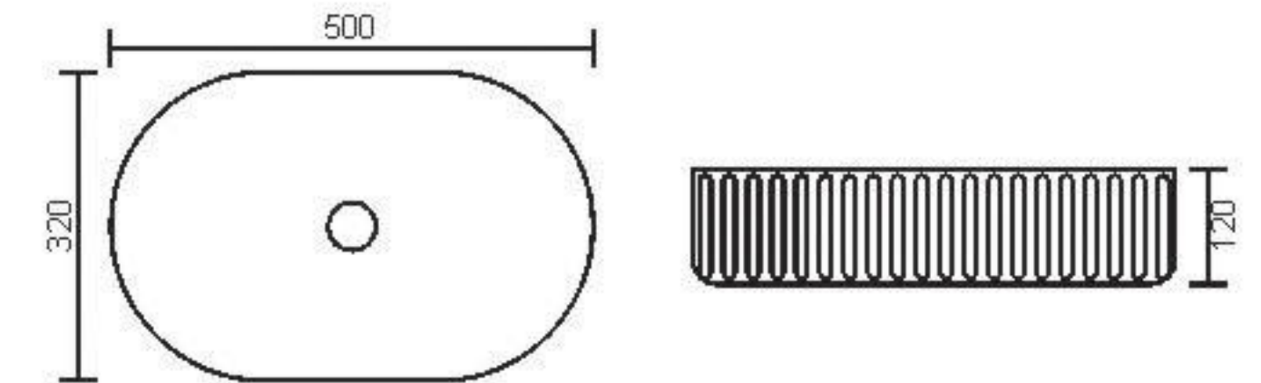
RING Size : 500 x 320 x 120 mm | GLOSS WHITE Rs. 12,998.00
