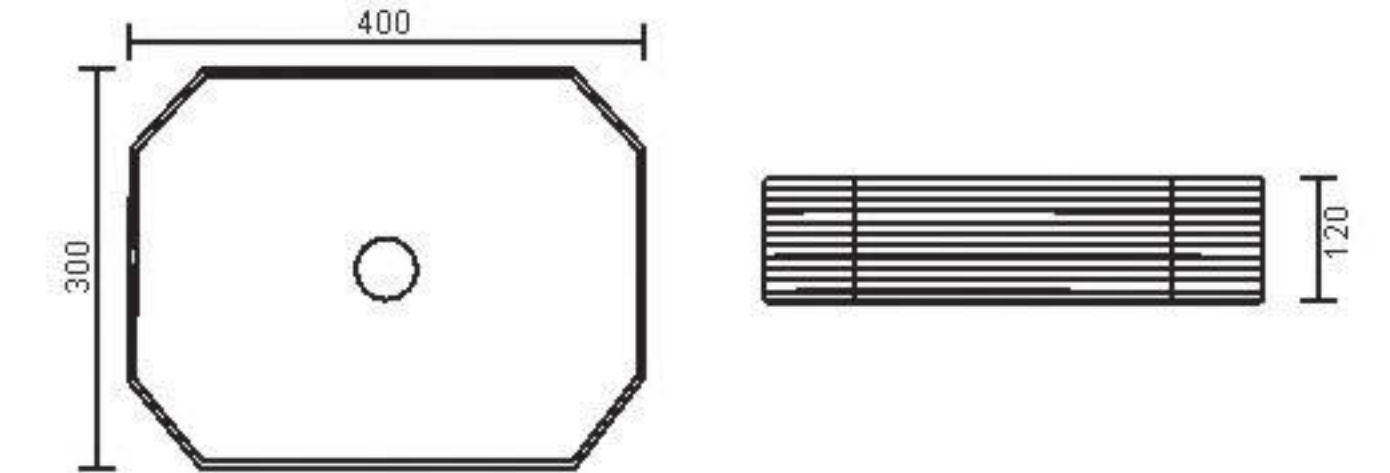
OLIO Size : 400 x 300 x 120 mm | GLOSS WHITE Rs. 8,998.00
