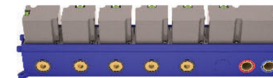
RETRO MAXX 5+ (Body) Diverter Body with 5 Outlets
